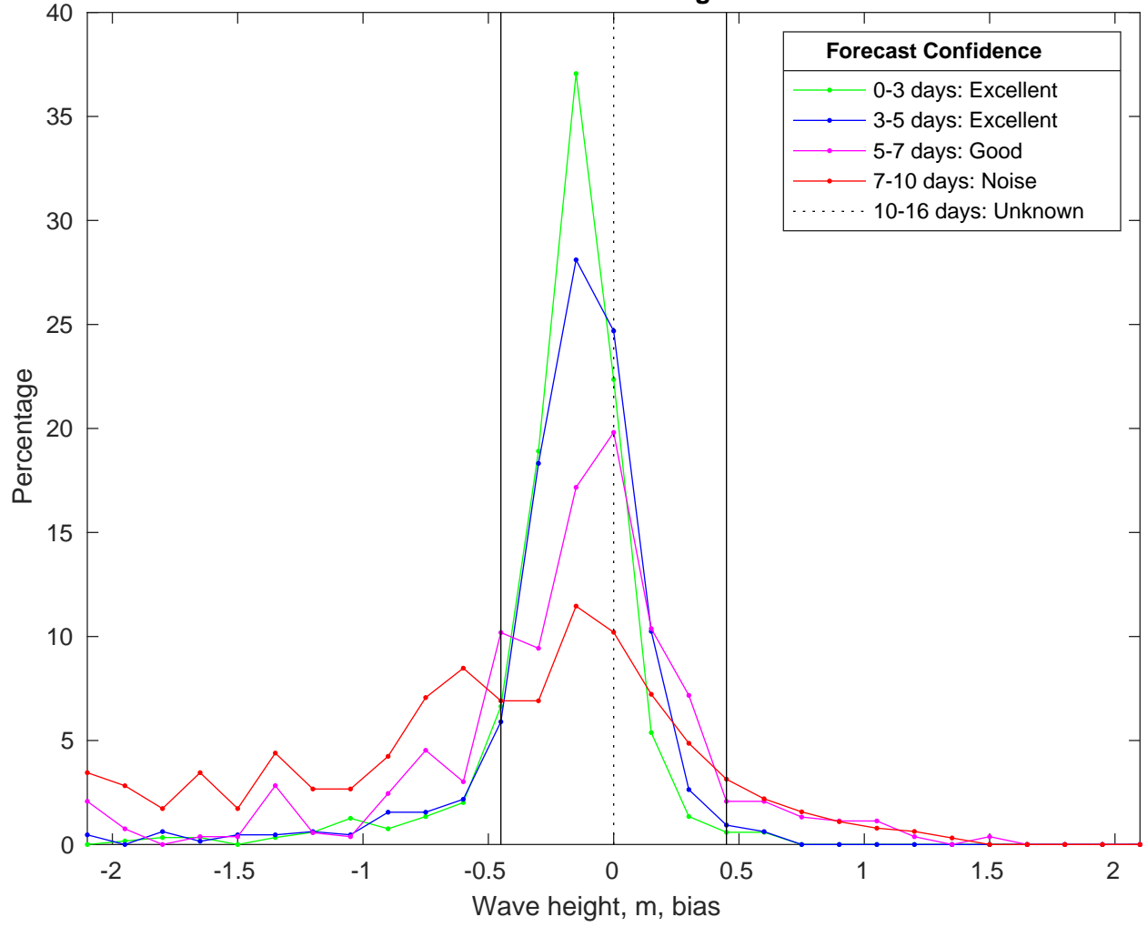
NDBC 42040 vs CMEMSWaves Bias Histogram: 18-Jan-2025
