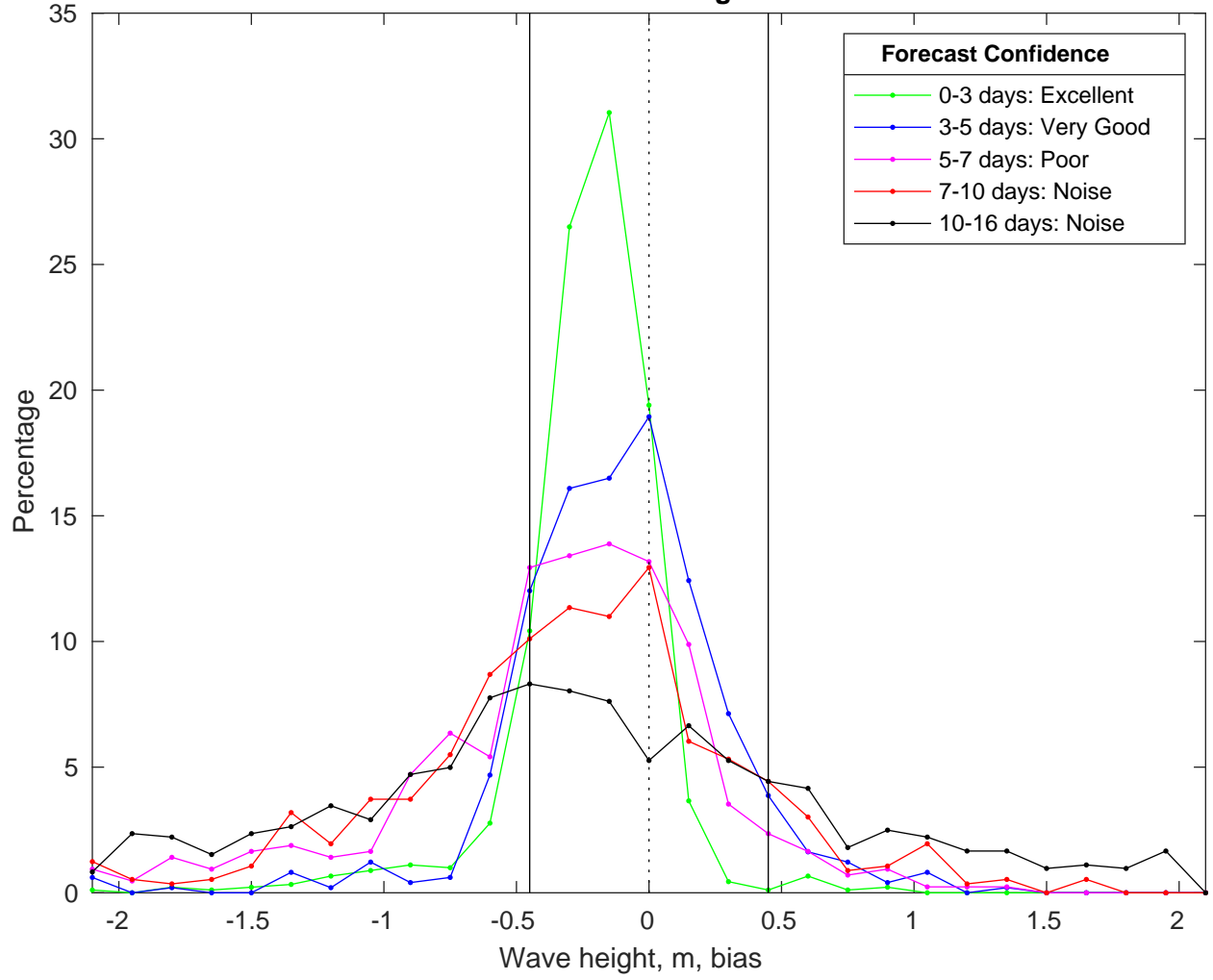
NDBC 42040 vs GFSWaves Bias Histogram: 18-Jan-2025
