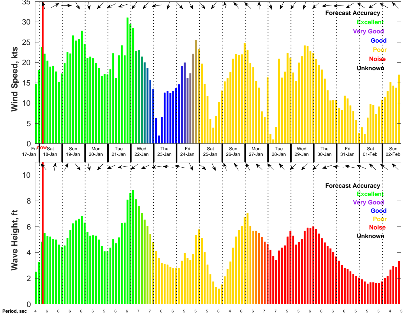
Wind & Wave Forecast for NDBC 42040 from 17-Jan-2025 19:00:00 to 02-Feb-2025 19:00:00
