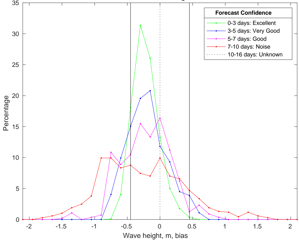
NDBC 42092 vs CMEMSWaves Bias Histogram: 18-Jan-2025
