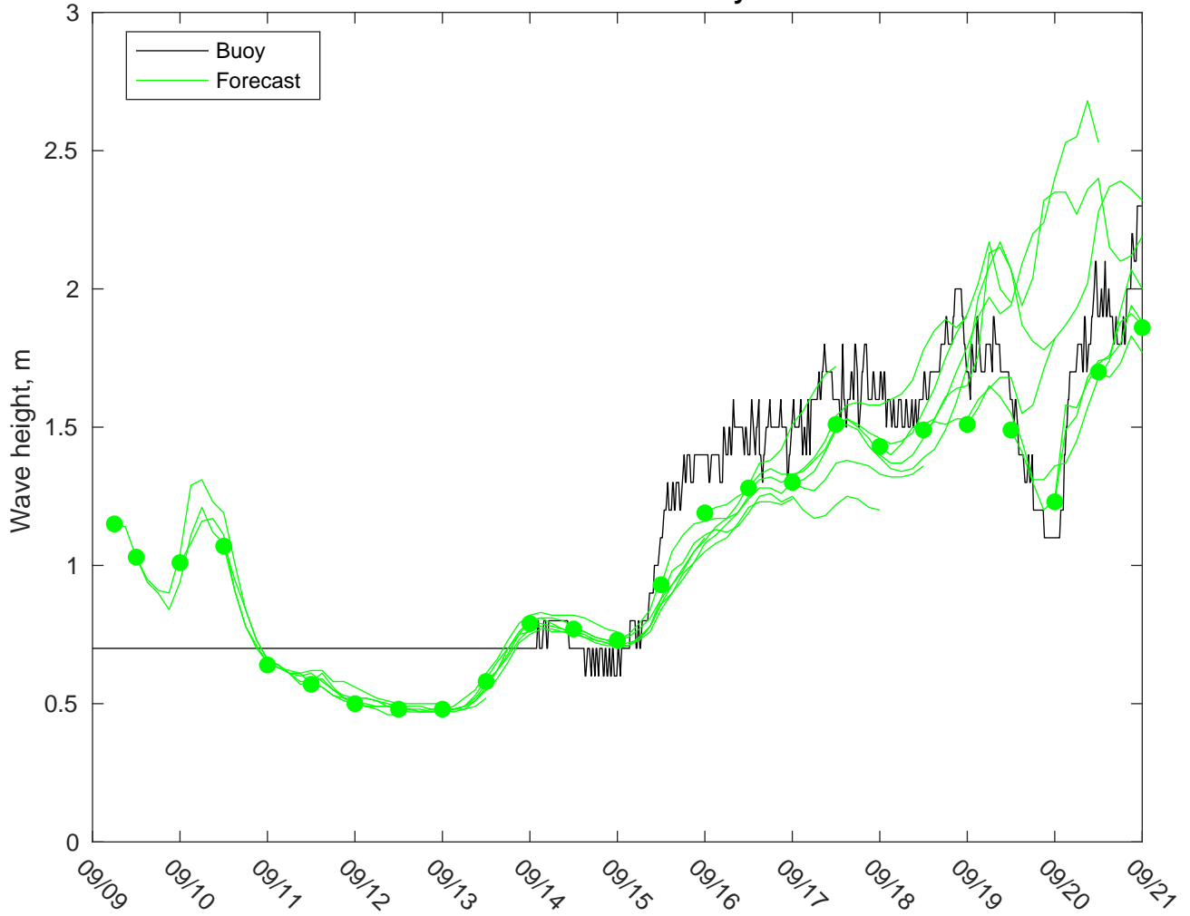
NDBC 44025 vs GFSWaves: 0 to 3 day forecast
