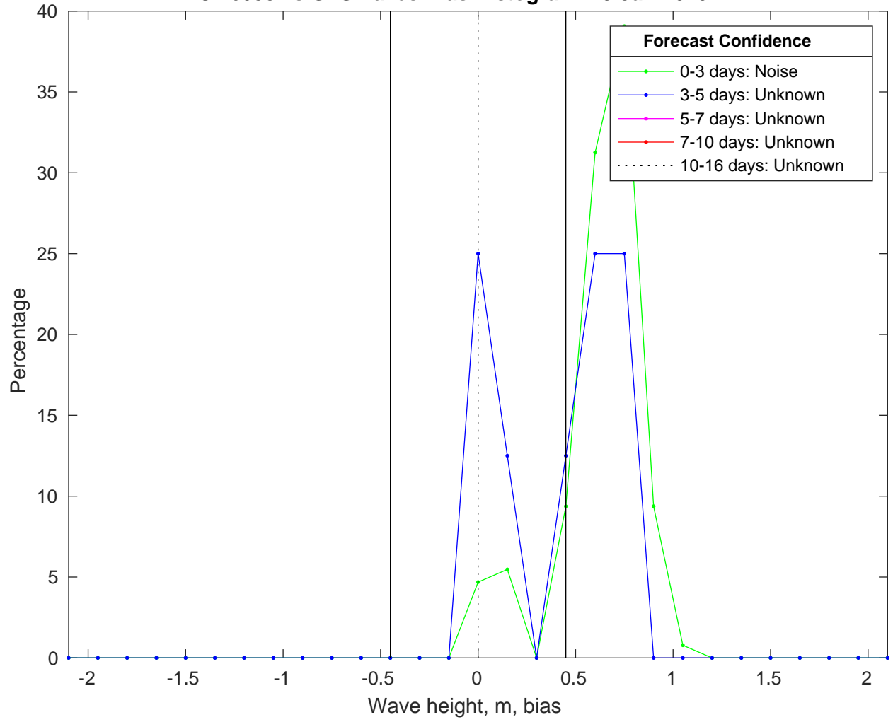
NDBC 46053 vs GFSWaves Bias Histogram: 18-Jan-2025
