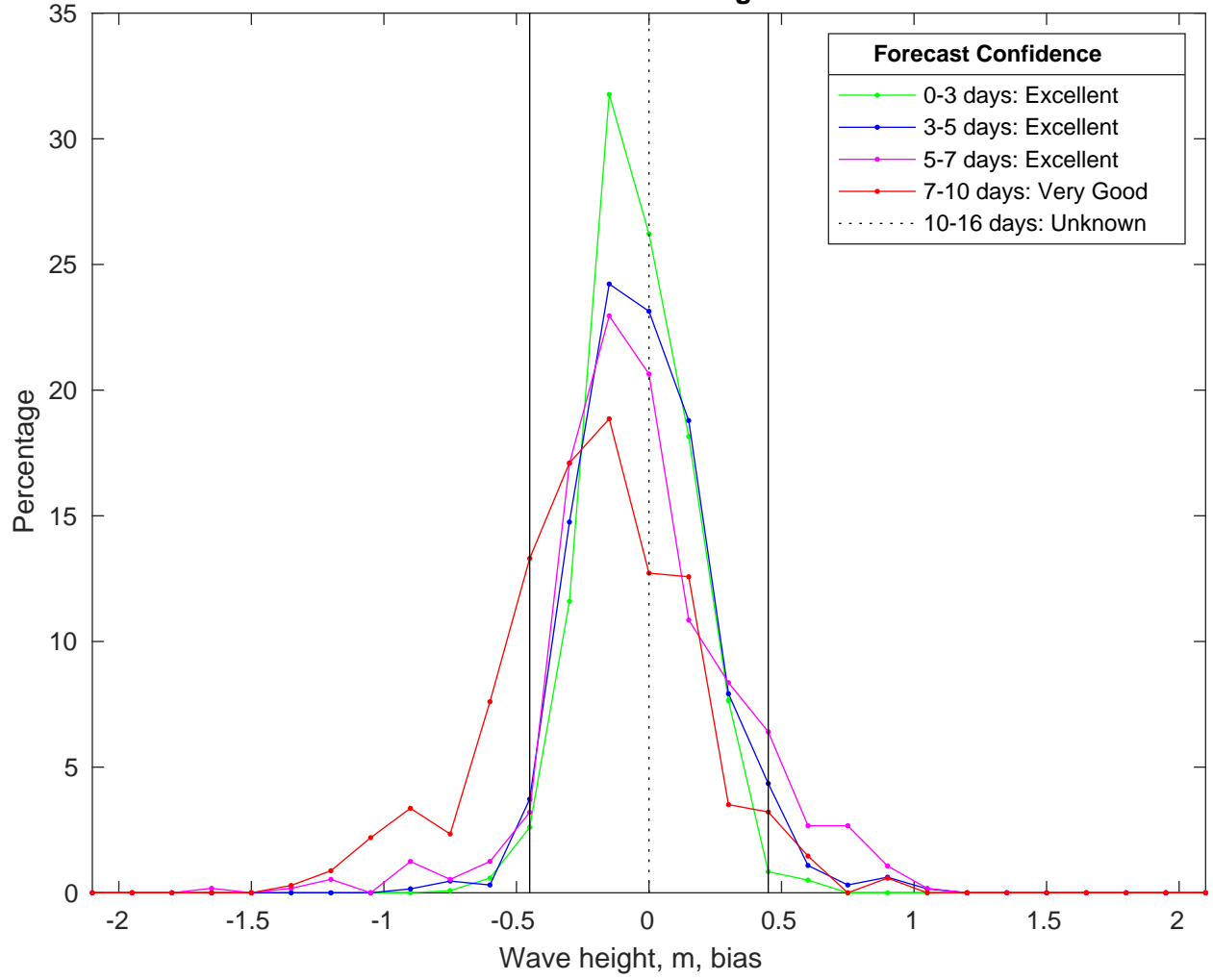
NDBC 46054 vs CMEMSWaves Bias Histogram: 18-Jan-2025
