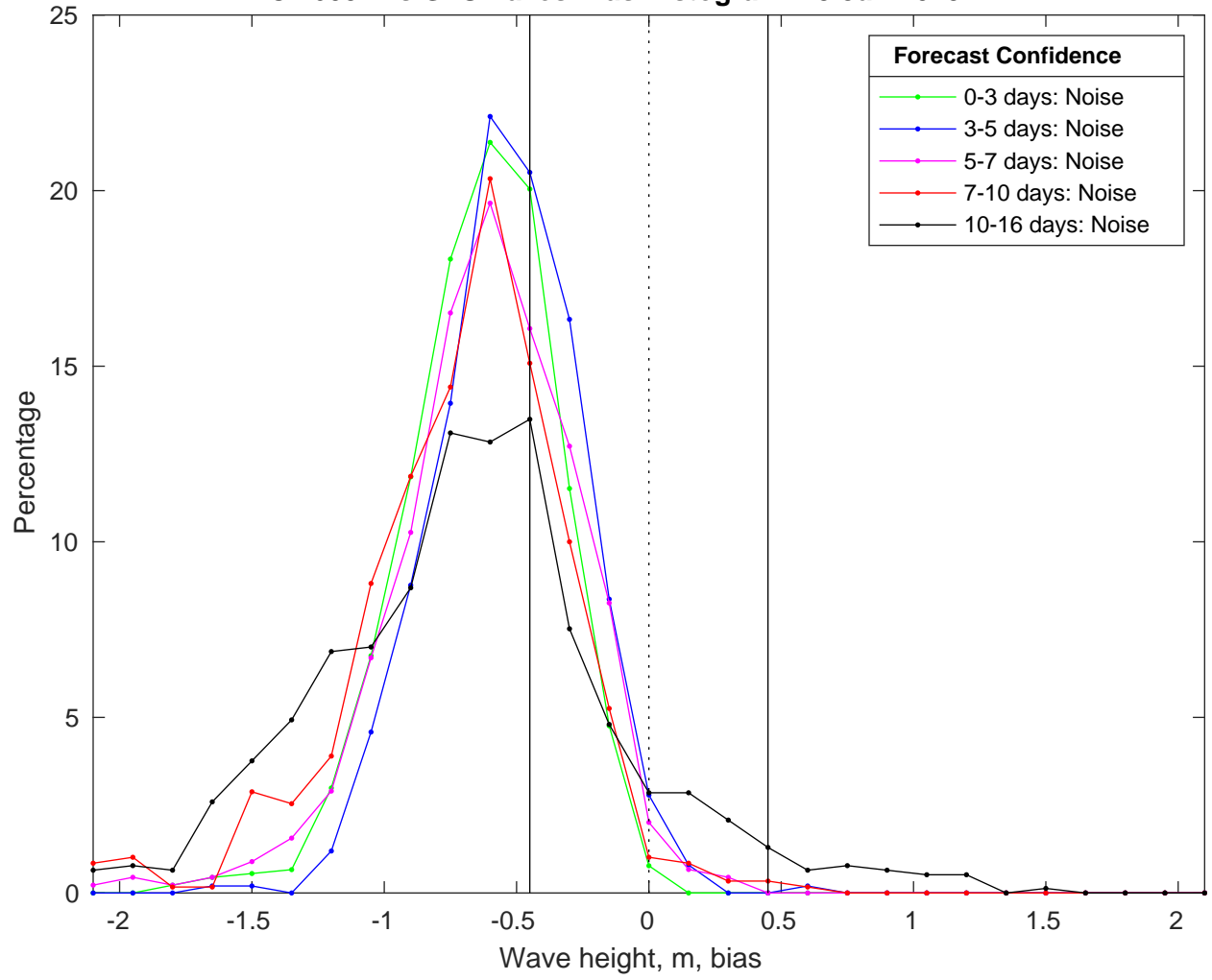
NDBC 46054 vs GFSWaves Bias Histogram: 18-Jan-2025
