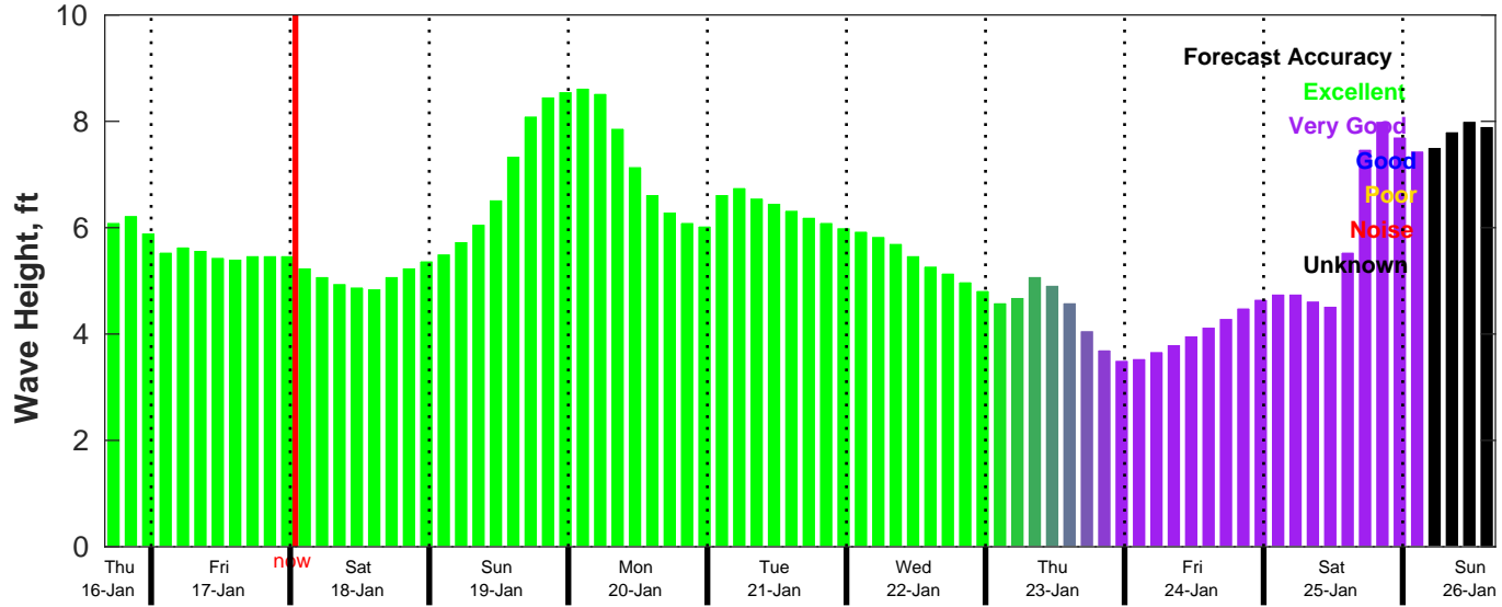
CMEMS Wave Forecast for NDBC 46054 from 16-Jan-2025 16:00:00 to 26-Jan-2025 16:00:00
