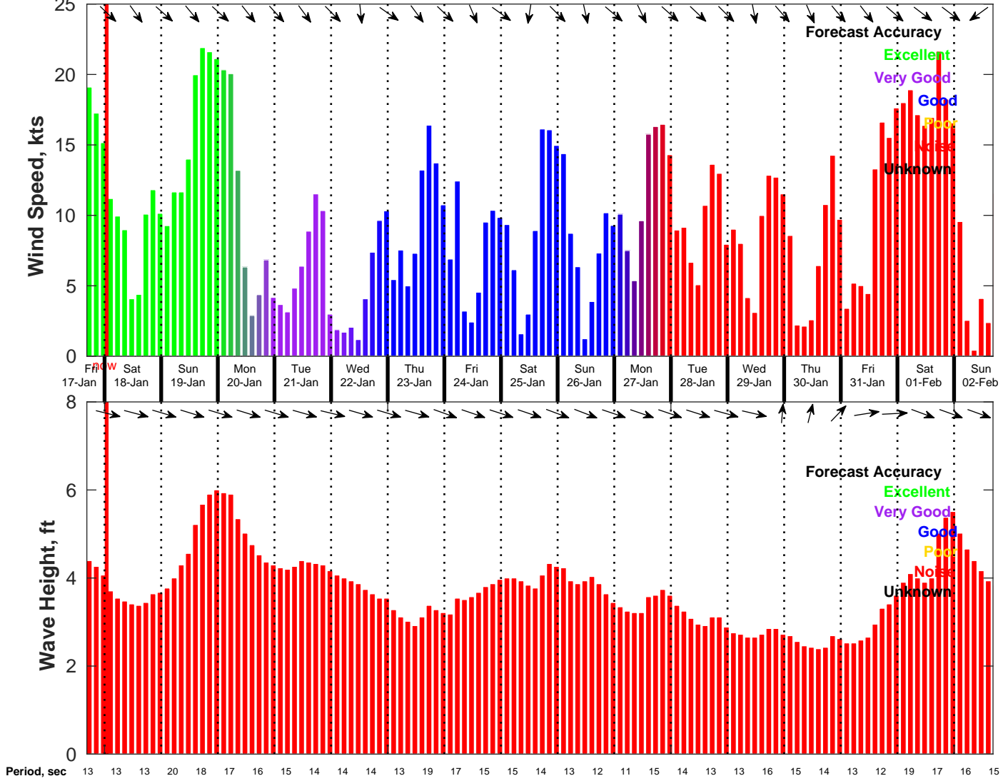
Wind & Wave Forecast for NDBC 46054 from 17-Jan-2025 16:00:00 to 02-Feb-2025 16:00:00
