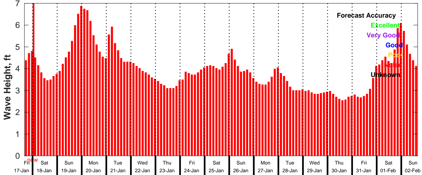
GFS Wave Forecast for NDBC 46069 from 17-Jan-2025 16:00:00 to 02-Feb-2025 16:00:00
