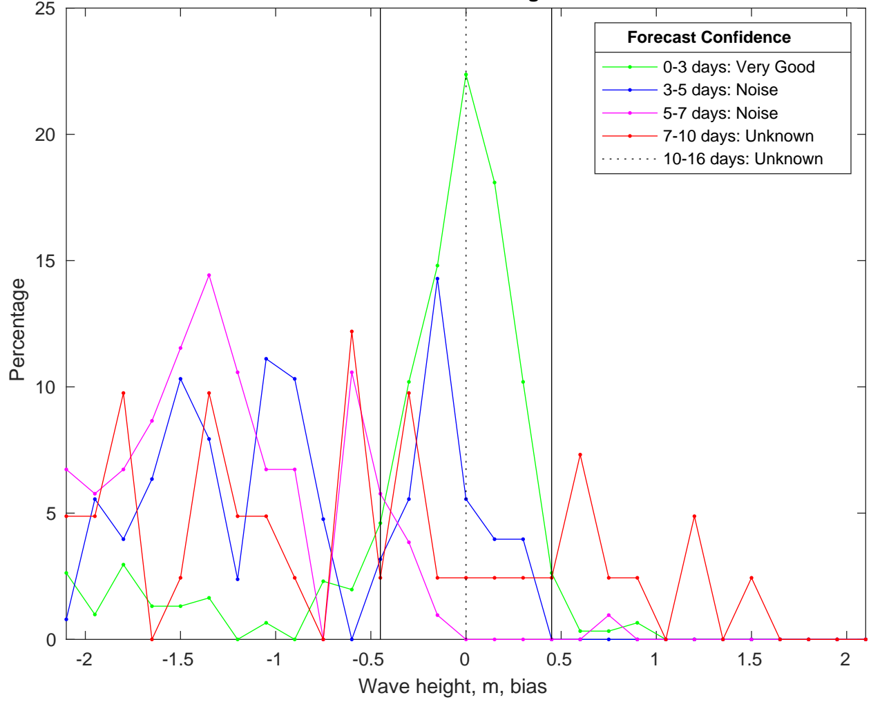
NDBC 46246 vs CMEMSWaves Bias Histogram: 18-Jan-2025
