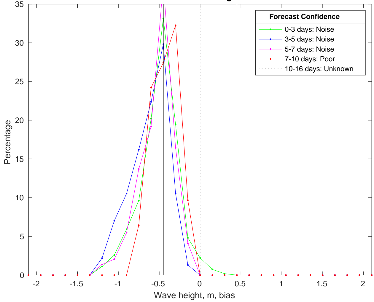
NDBC 51209 vs CMEMSWaves Bias Histogram: 18-Jan-2025
