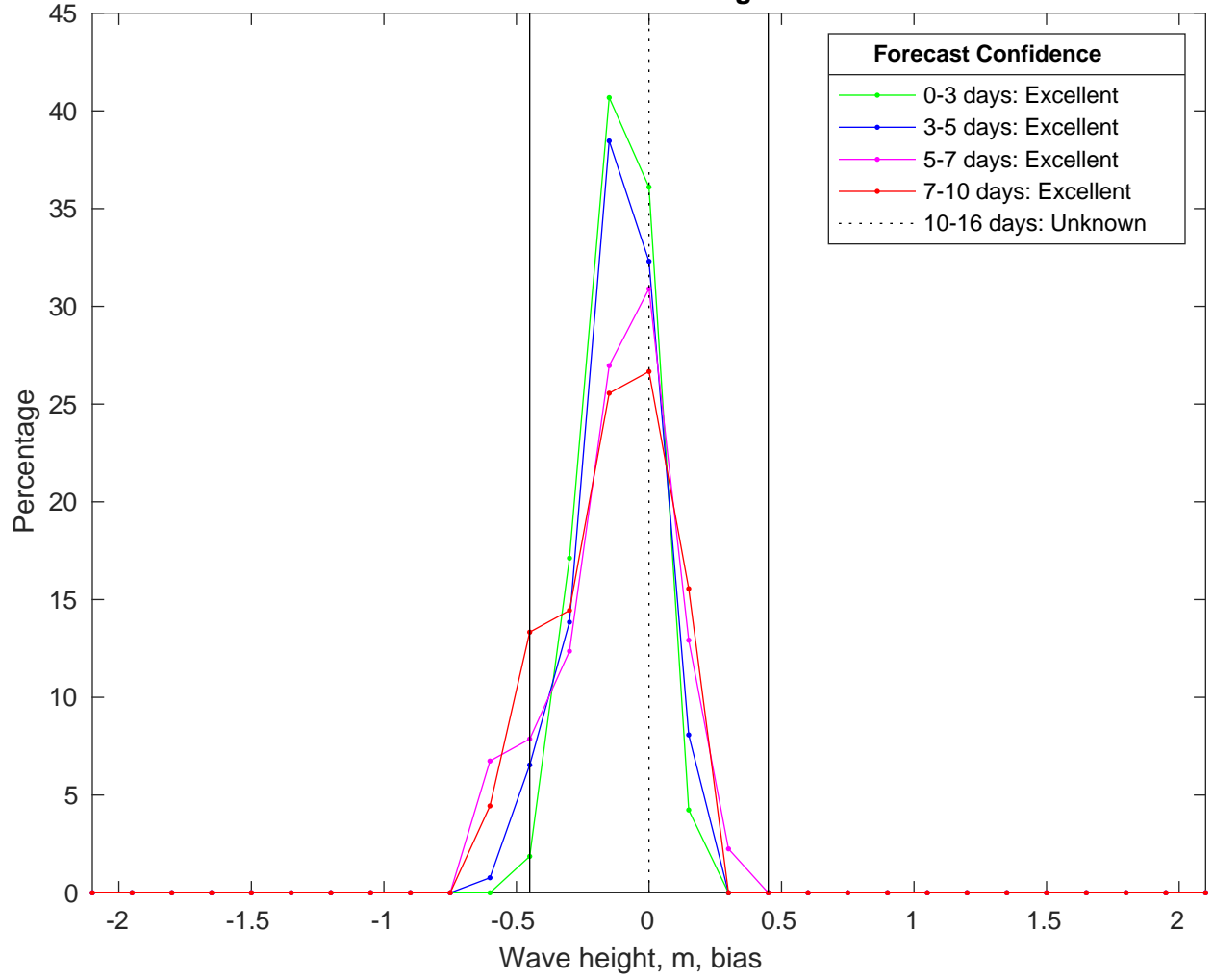
NDBC 52211 vs CMEMSWaves Bias Histogram: 18-Jan-2025
