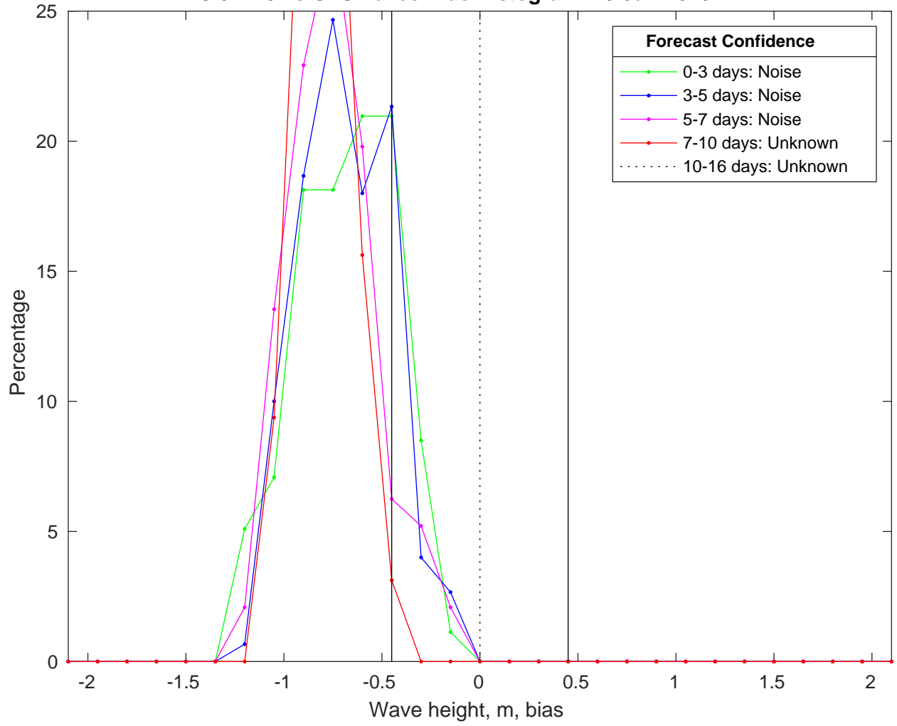
NDBC 52213 vs GFSWaves Bias Histogram: 18-Jan-2025
