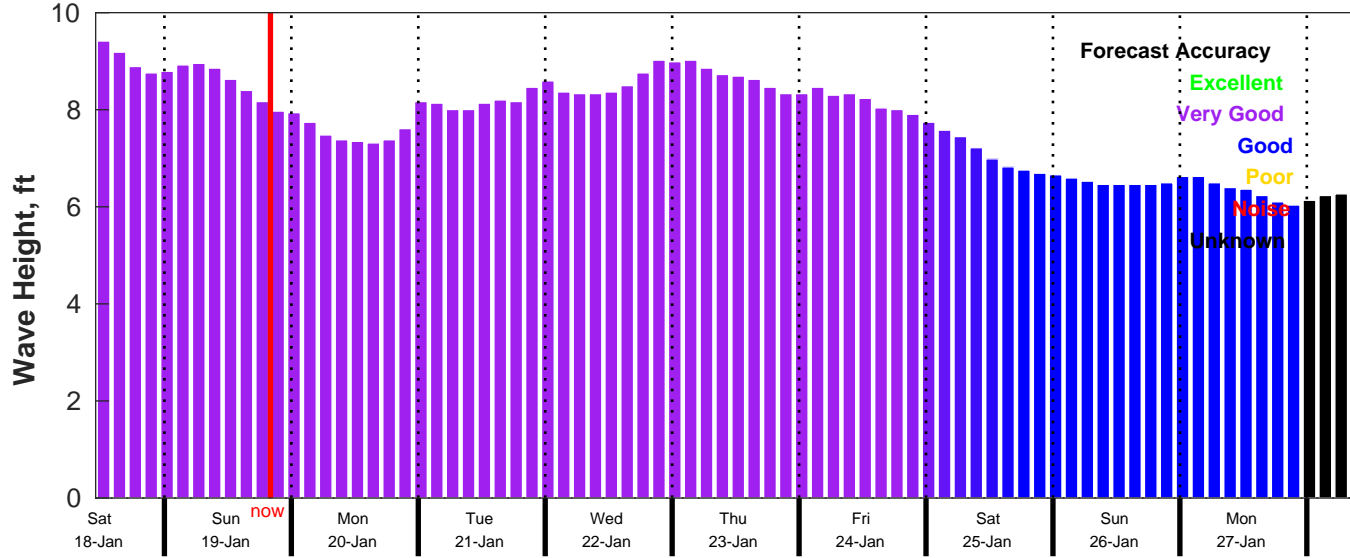
CMEMS Wave Forecast for NDBC 52213 from 17-Jan-2025 11:00:00 to 27-Jan-2025 11:00:00
