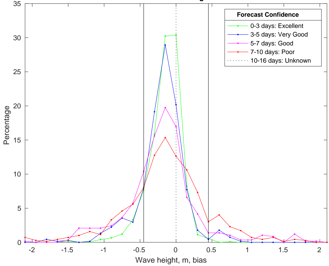
NDBC 41004 vs CMEMSWaves Bias Histogram: 19-Jan-2025
