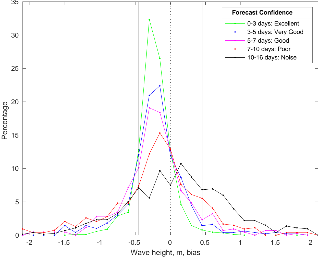
NDBC 41004 vs GFSWaves Bias Histogram: 19-Jan-2025
