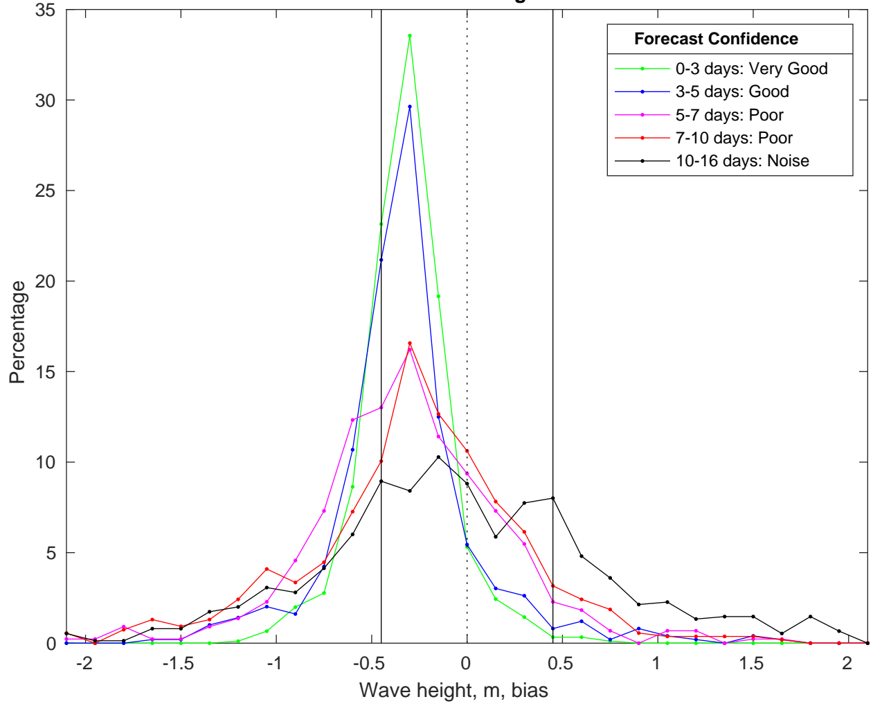
NDBC 41013 vs GFSWaves Bias Histogram: 19-Jan-2025
