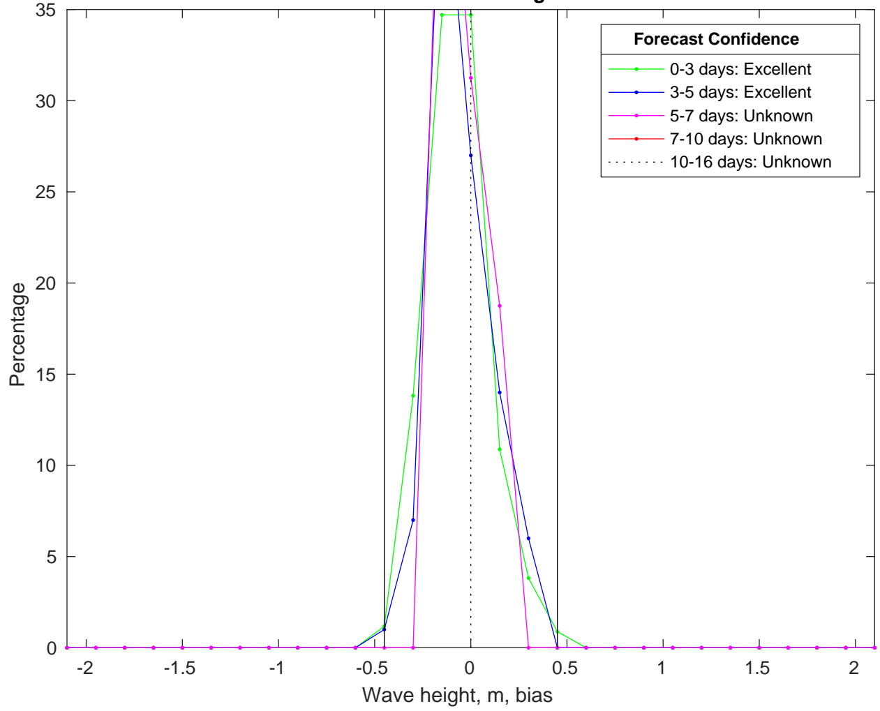
NDBC 41040 vs CMEMSWaves Bias Histogram: 19-Jan-2025
