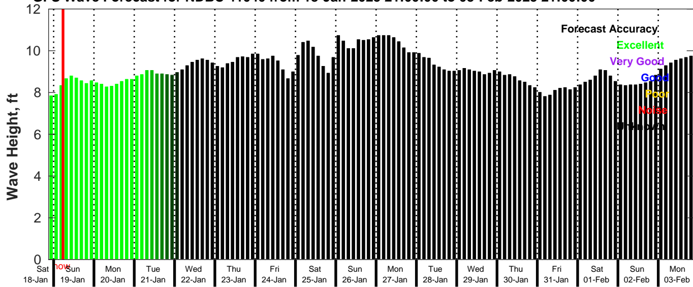
GFS Wave Forecast for NDBC 41040 from 18-Jan-2025 21:00:00 to 03-Feb-2025 21:00:00
