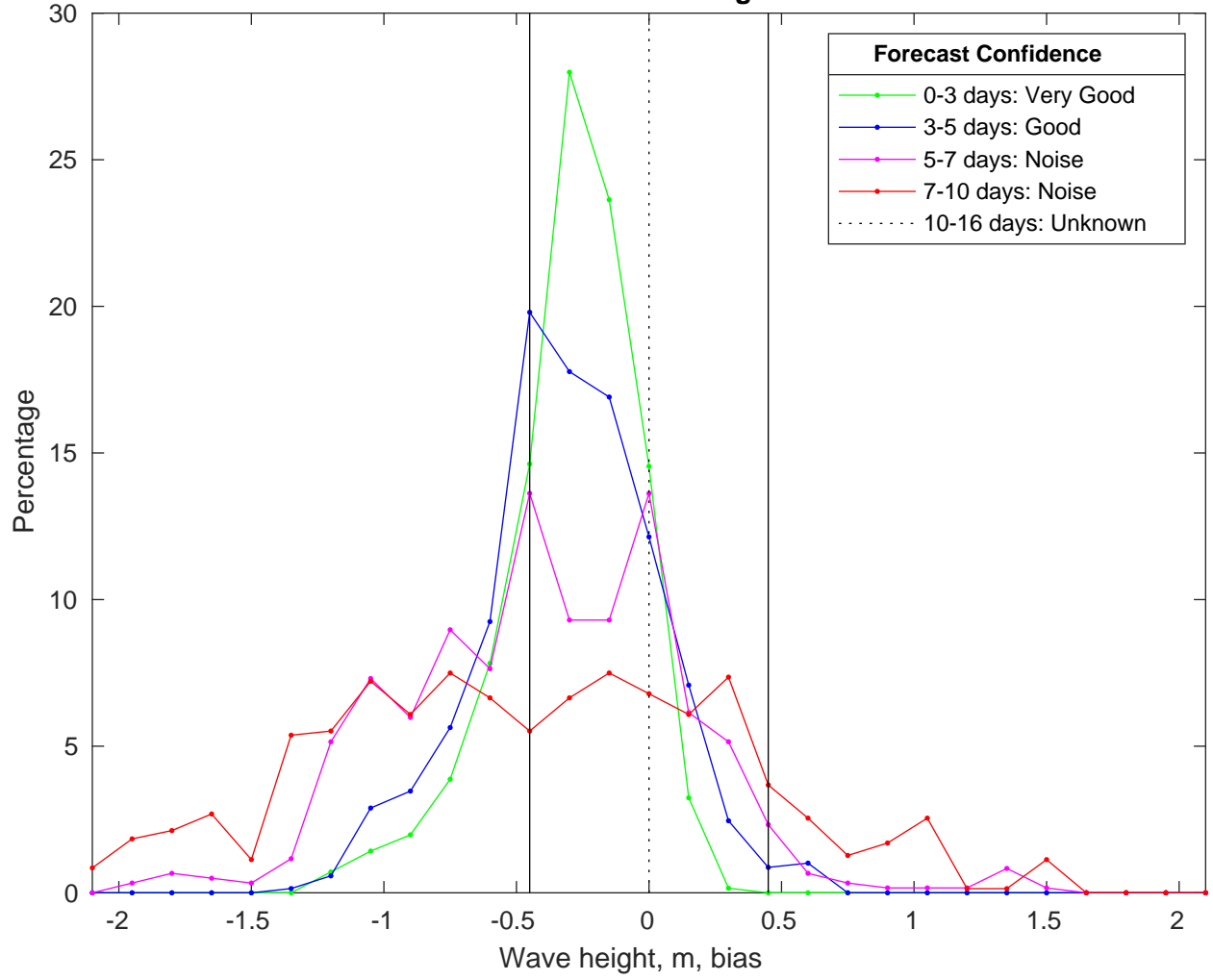
NDBC 42019 vs CMEMSWaves Bias Histogram: 19-Jan-2025
