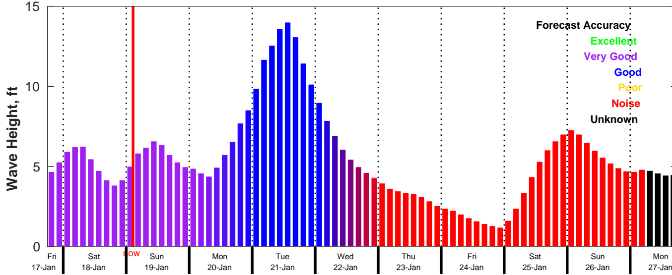
CMEMS Wave Forecast for NDBC 42019 from 17-Jan-2025 18:00:00 to 27-Jan-2025 18:00:00
