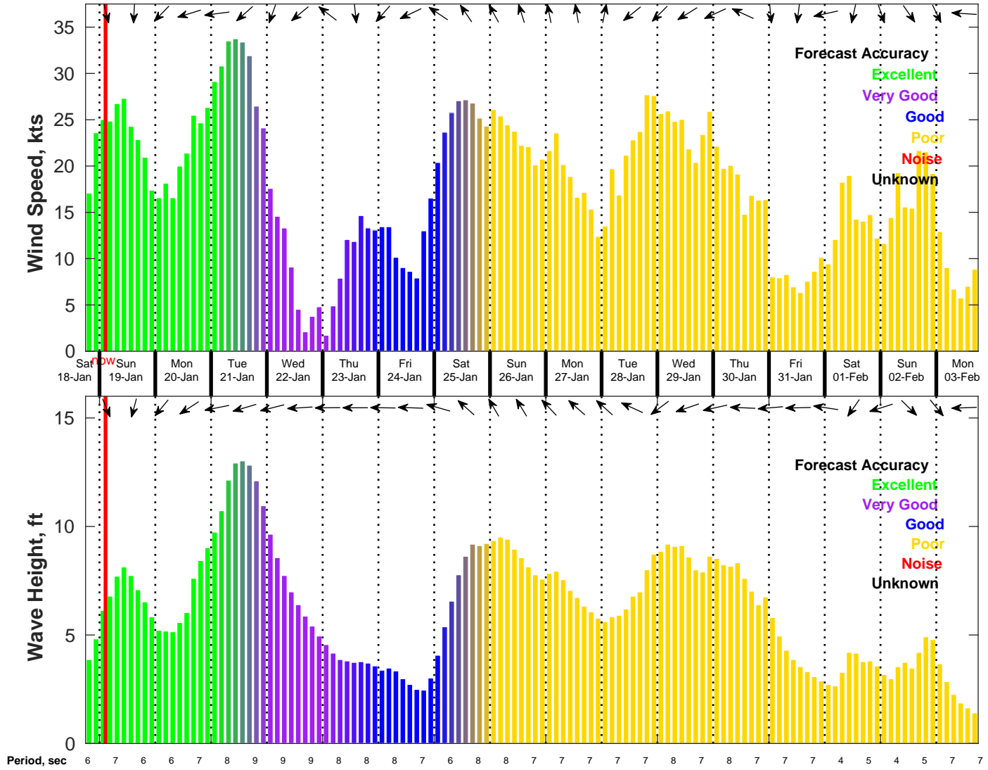
Wind & Wave Forecast for NDBC 42019 from 18-Jan-2025 18:00:00 to 03-Feb-2025 18:00:00
