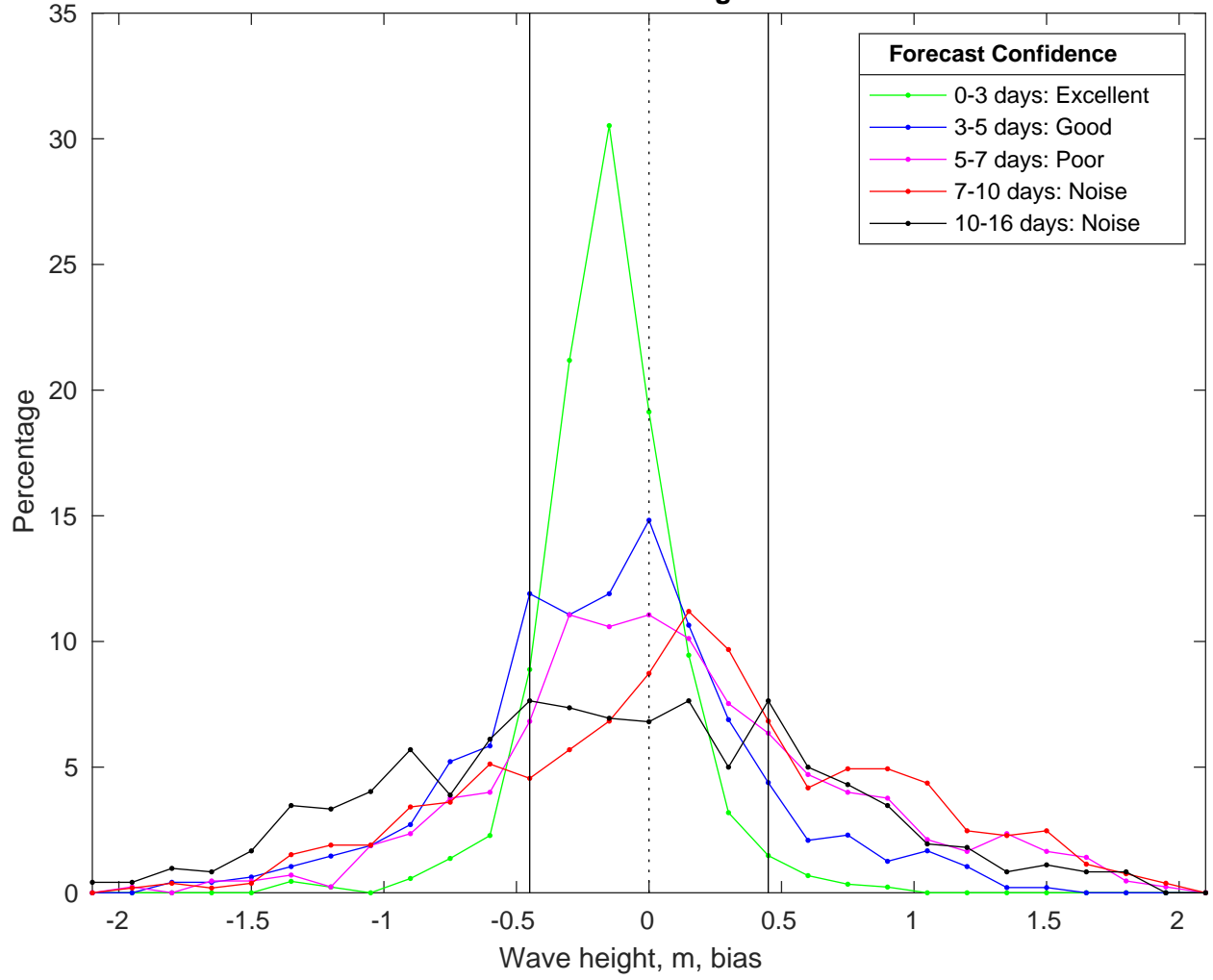
NDBC 42020 vs GFSWaves Bias Histogram: 19-Jan-2025
