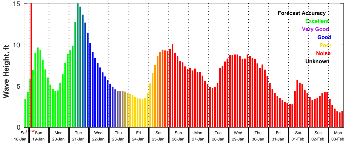
GFS Wave Forecast for NDBC 42020 from 18-Jan-2025 18:00:00 to 03-Feb-2025 18:00:00
