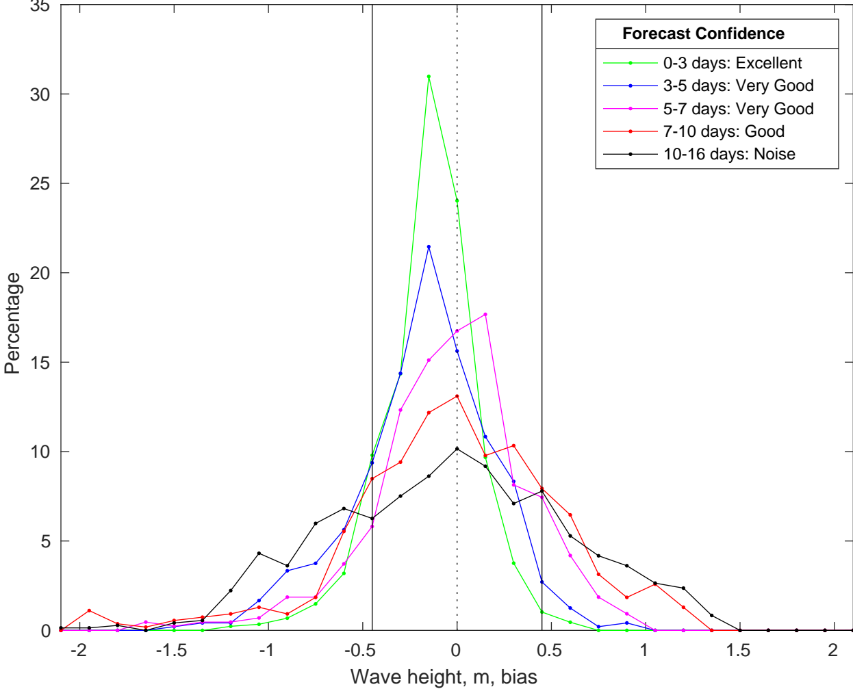
NDBC 42035 vs GFSWaves Bias Histogram: 19-Jan-2025
