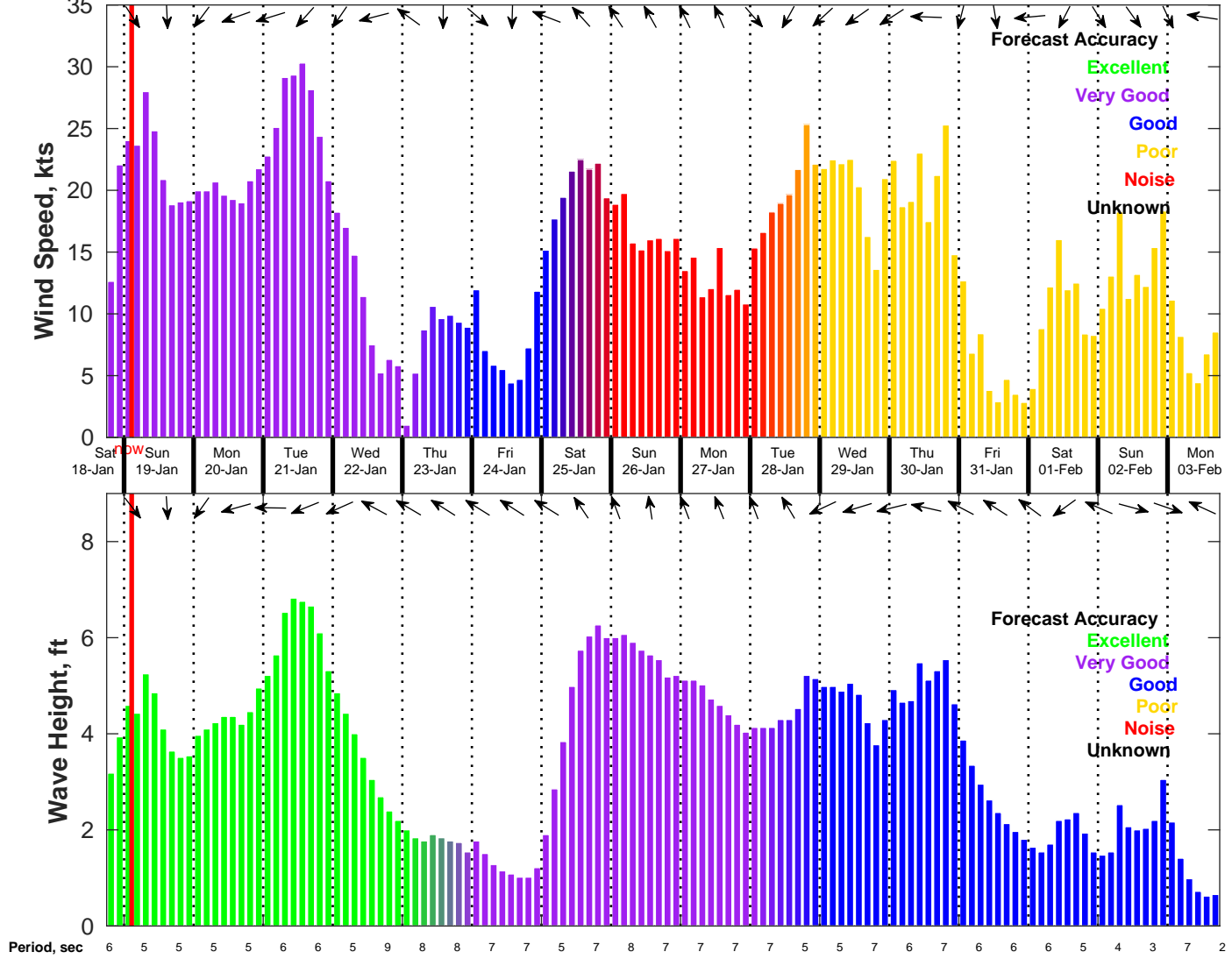
Wind & Wave Forecast for NDBC 42035 from 18-Jan-2025 18:00:00 to 03-Feb-2025 18:00:00
