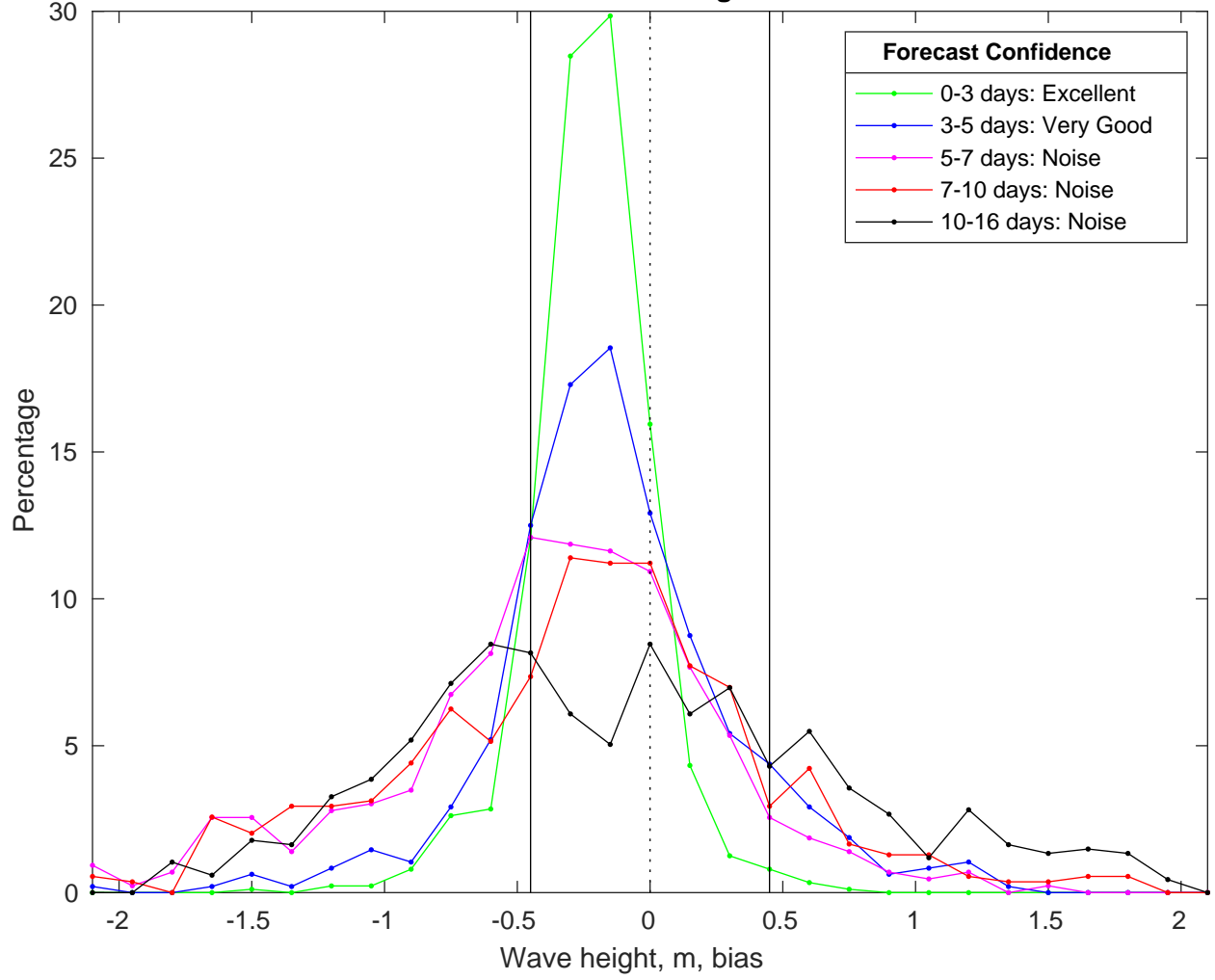
NDBC 42036 vs GFSWaves Bias Histogram: 19-Jan-2025
