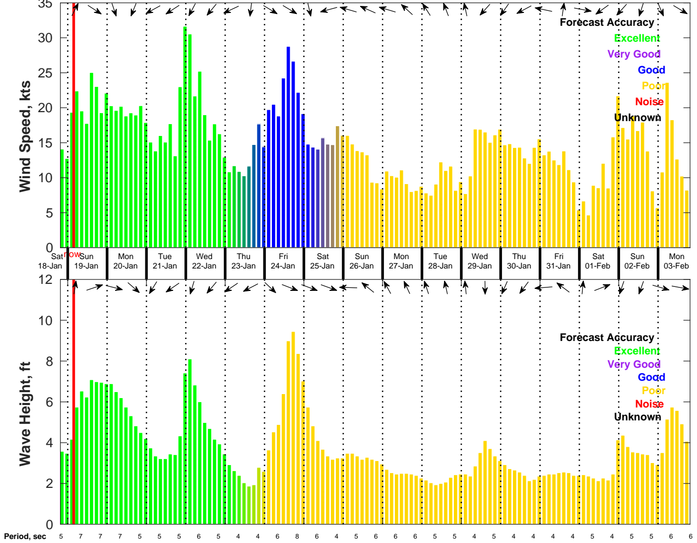
Wind & Wave Forecast for NDBC 42036 from 18-Jan-2025 19:00:00 to 03-Feb-2025 19:00:00
