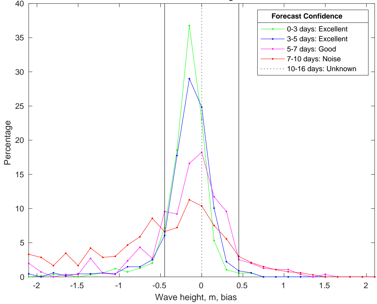
NDBC 42040 vs CMEMSWaves Bias Histogram: 19-Jan-2025
