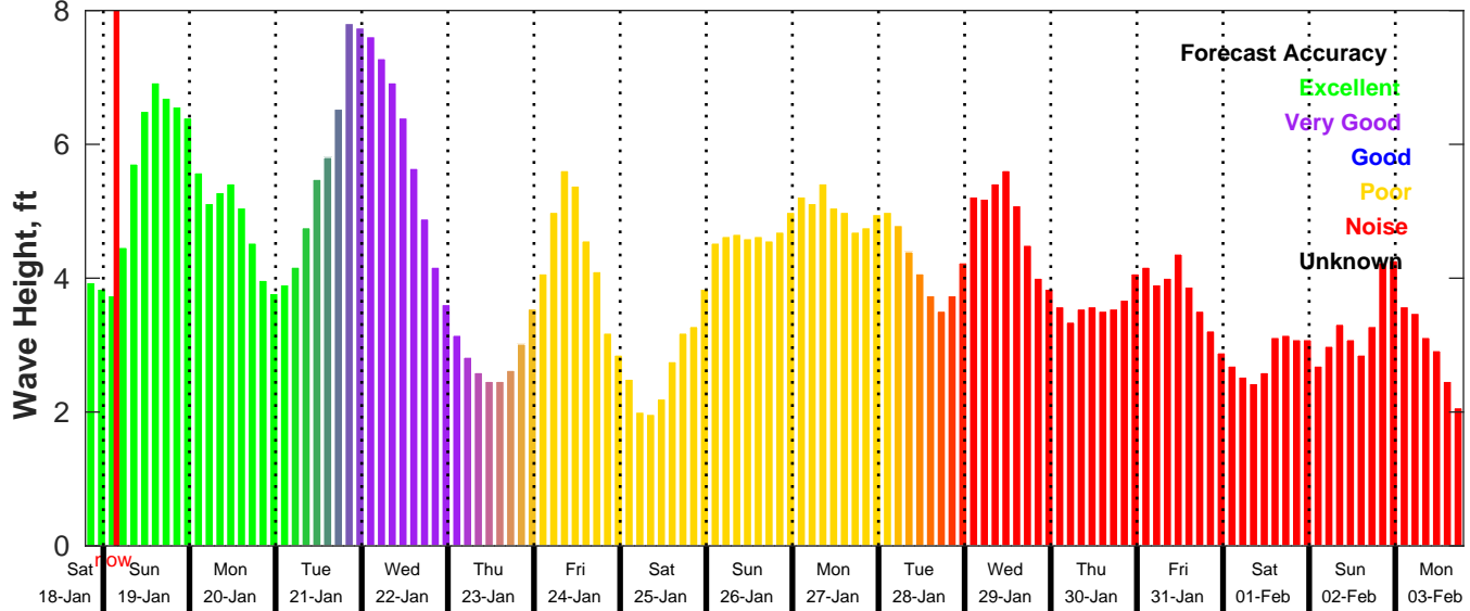
GFS Wave Forecast for NDBC 42040 from 18-Jan-2025 19:00:00 to 03-Feb-2025 19:00:00
