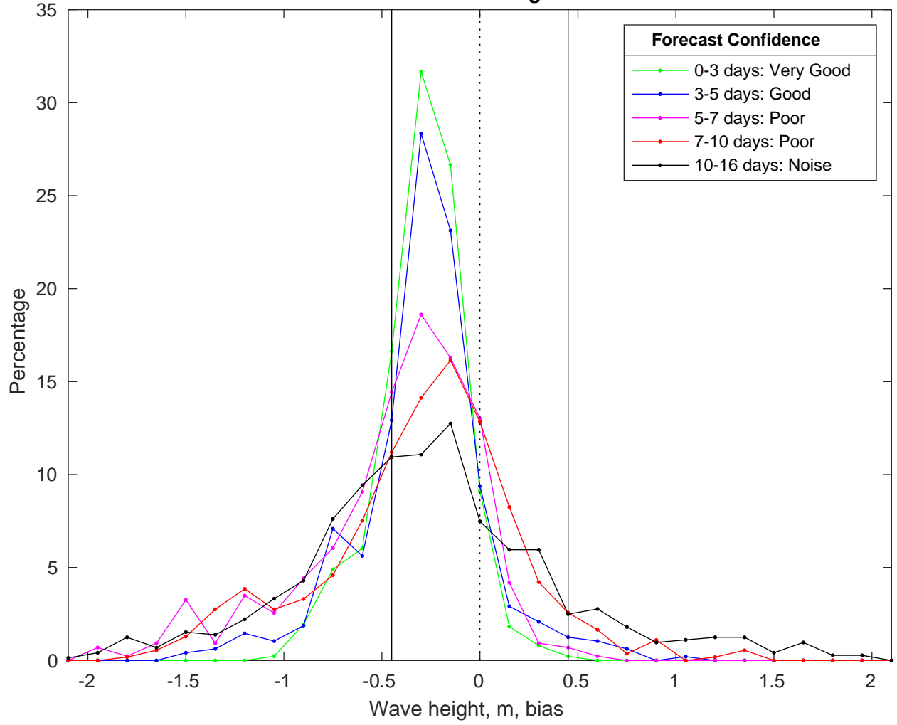
NDBC 42084 vs GFSWaves Bias Histogram: 19-Jan-2025
