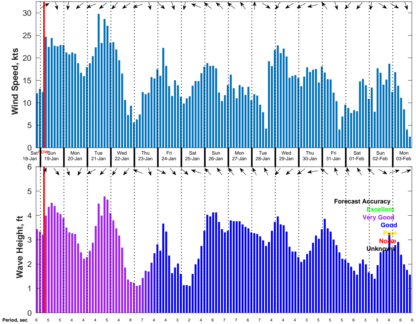
Wind & Wave Forecast for NDBC 42084 from 18-Jan-2025 19:00:00 to 03-Feb-2025 19:00:00
