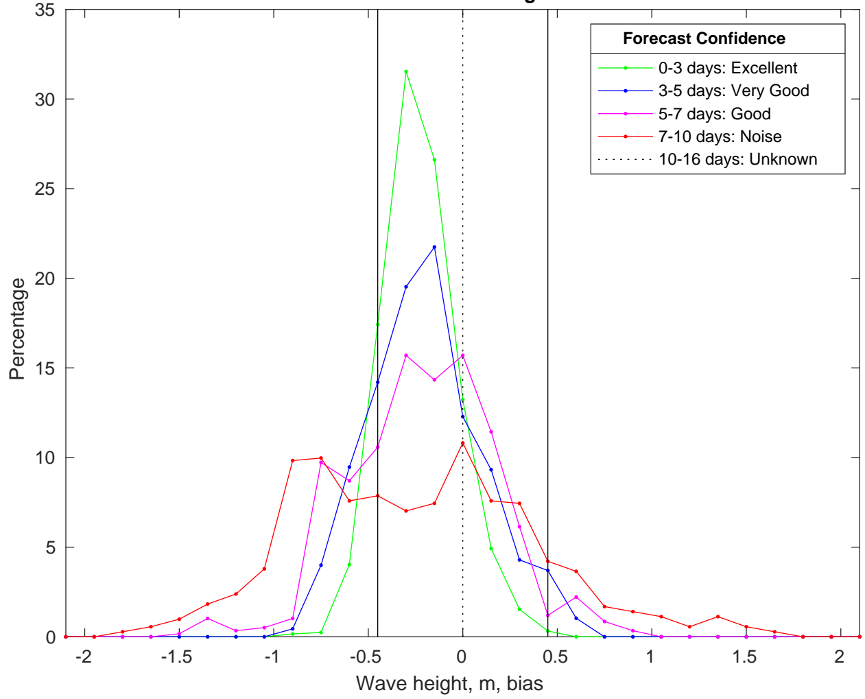
NDBC 42092 vs CMEMSWaves Bias Histogram: 19-Jan-2025
