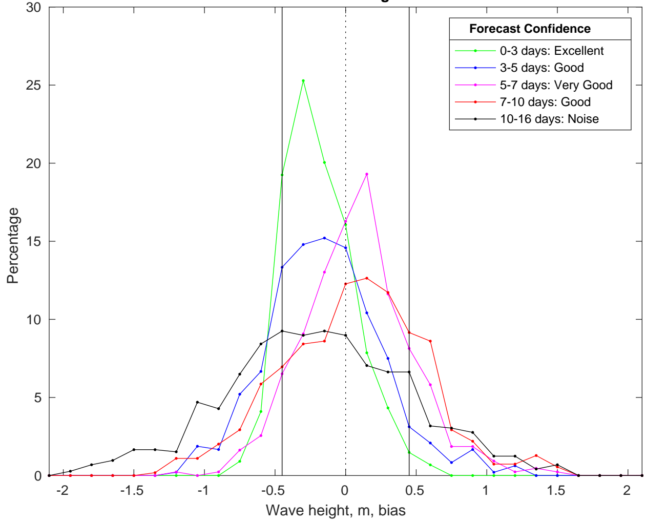
NDBC 42092 vs GFSWaves Bias Histogram: 19-Jan-2025
