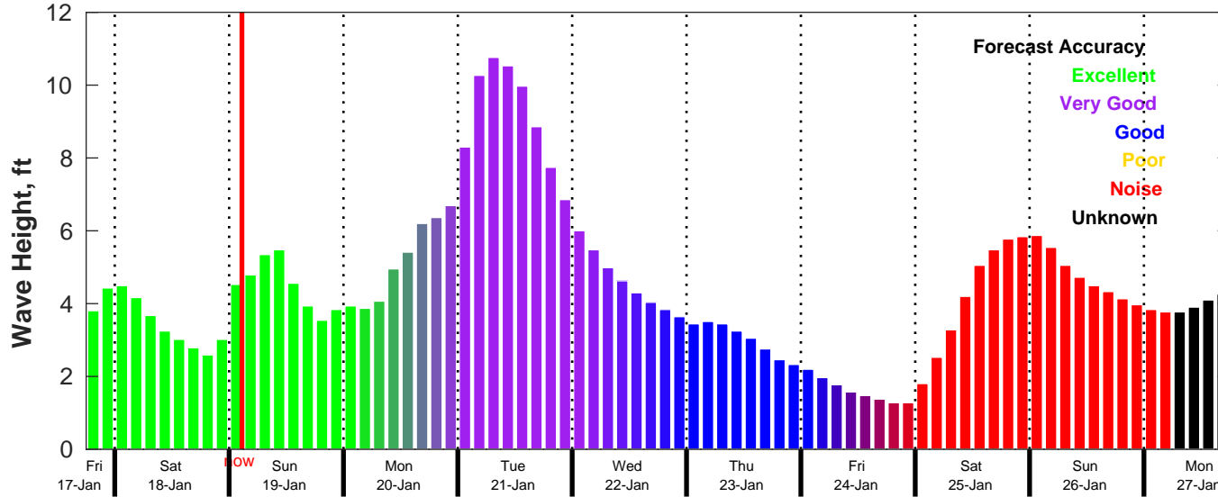
CMEMS Wave Forecast for NDBC 42092 from 17-Jan-2025 18:00:00 to 27-Jan-2025 18:00:00
