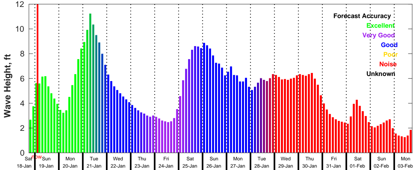
GFS Wave Forecast for NDBC 42092 from 18-Jan-2025 18:00:00 to 03-Feb-2025 18:00:00
