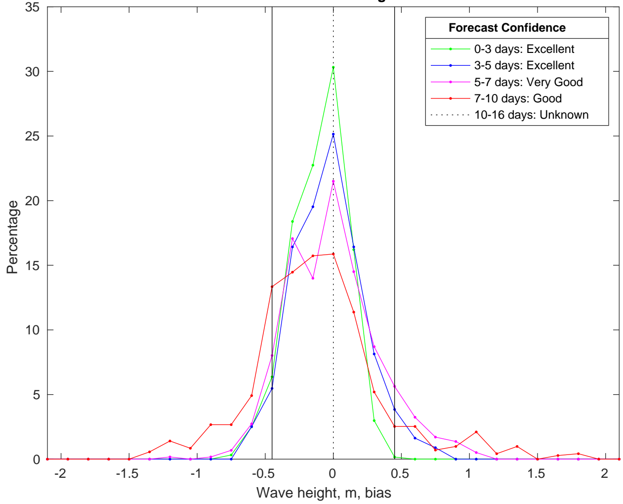
NDBC 46011 vs CMEMSWaves Bias Histogram: 19-Jan-2025
