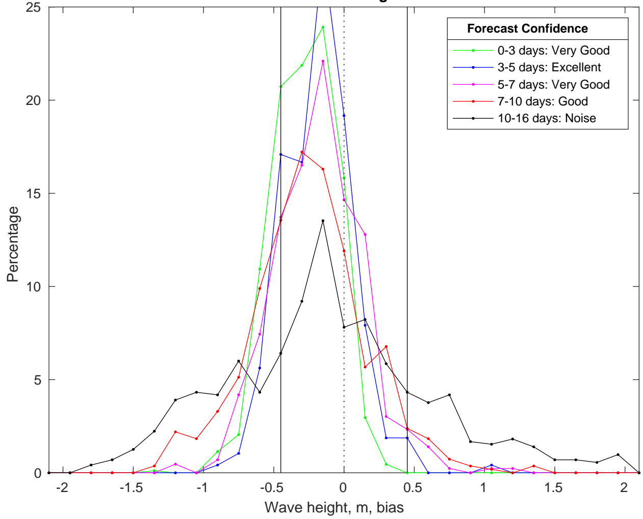
NDBC 46011 vs GFSWaves Bias Histogram: 19-Jan-2025
