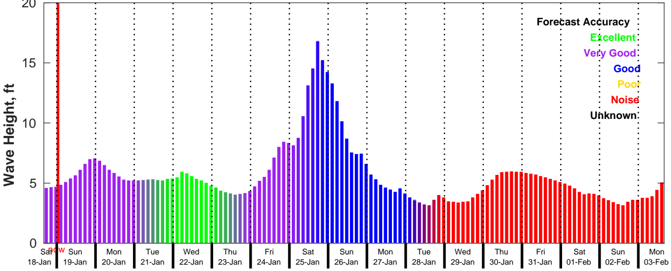
GFS Wave Forecast for NDBC 46011 from 18-Jan-2025 16:00:00 to 03-Feb-2025 16:00:00
