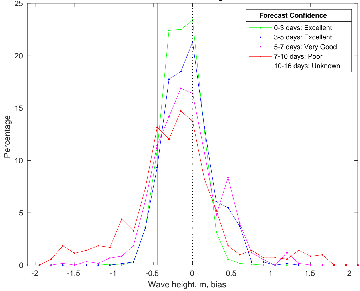
NDBC 46028 vs CMEMSWaves Bias Histogram: 19-Jan-2025
