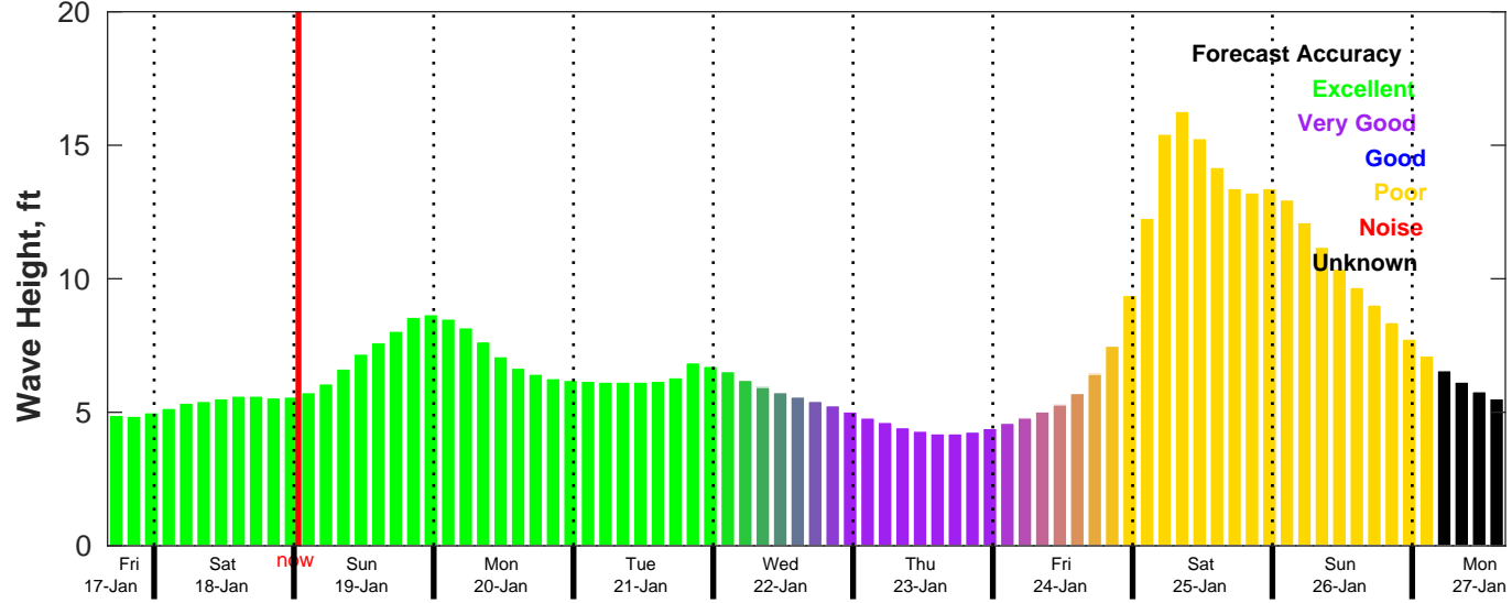
CMEMS Wave Forecast for NDBC 46028 from 17-Jan-2025 16:00:00 to 27-Jan-2025 16:00:00
