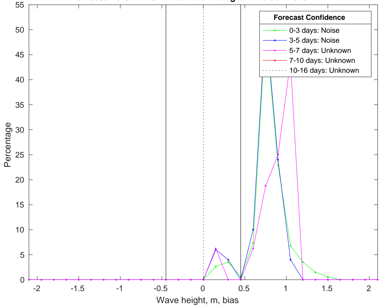
NDBC 46053 vs CMEMSWaves Bias Histogram: 19-Jan-2025
