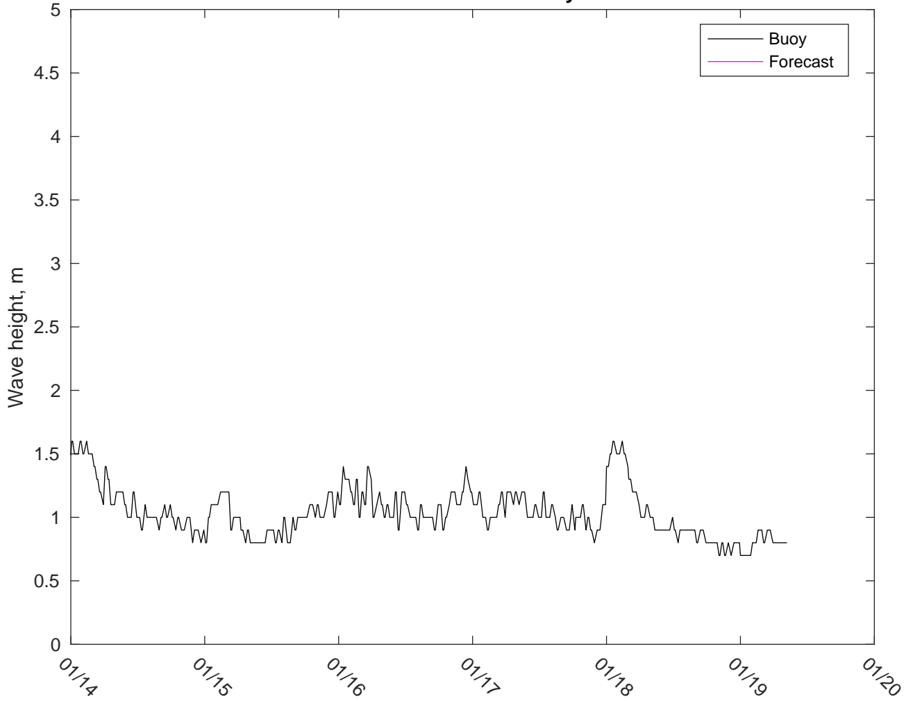
NDBC 46053 vs GFSWaves: 7 to 10 day forecast
