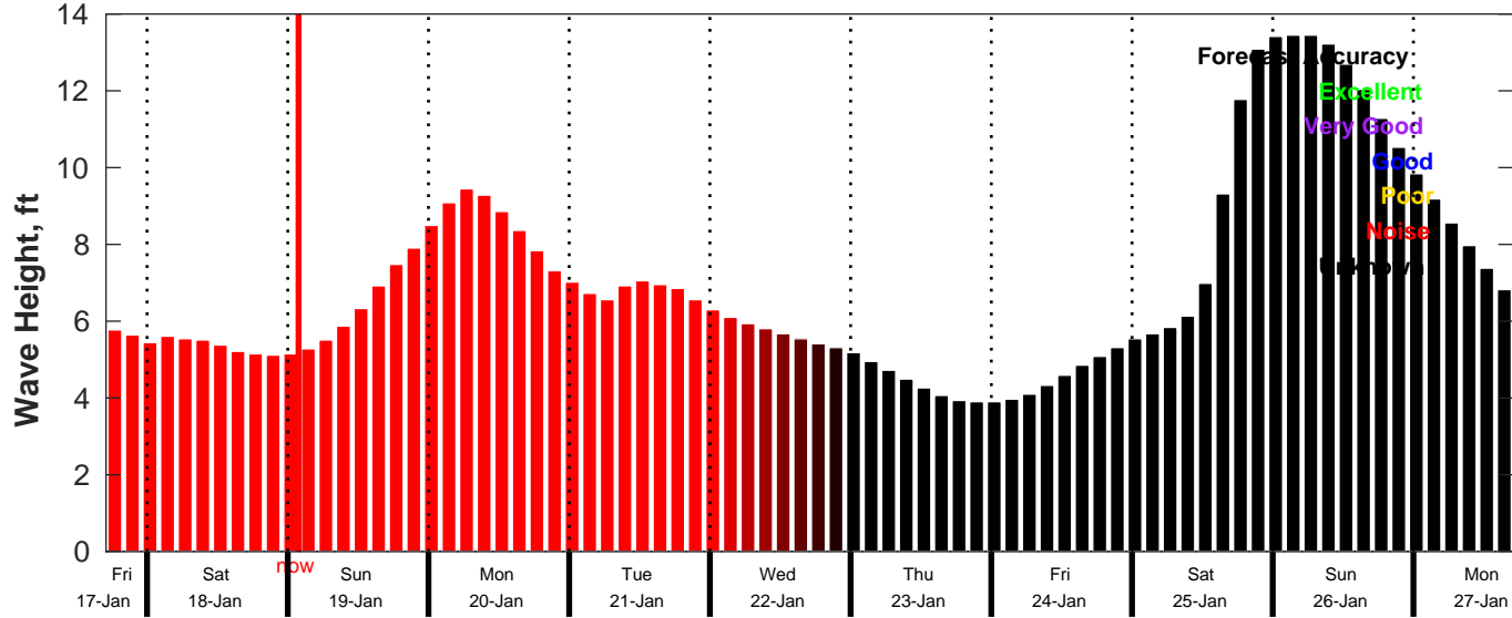
CMEMS Wave Forecast for NDBC 46053 from 17-Jan-2025 17:00:00 to 27-Jan-2025 17:00:00
