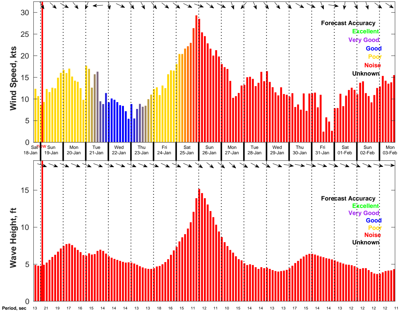
Wind & Wave Forecast for NDBC 46053 from 18-Jan-2025 17:00:00 to 03-Feb-2025 17:00:00
