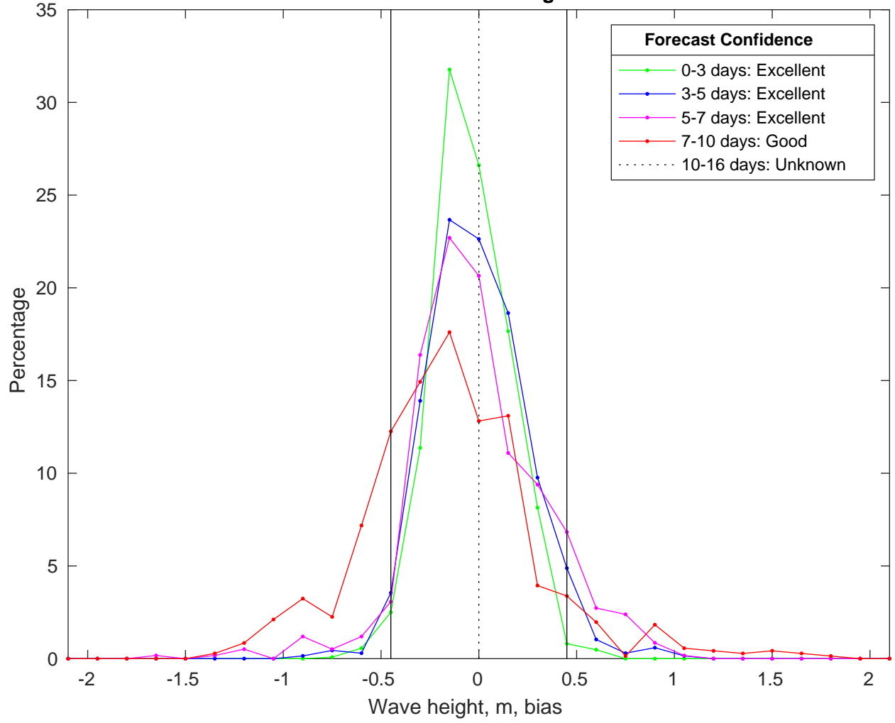
NDBC 46054 vs CMEMSWaves Bias Histogram: 19-Jan-2025
