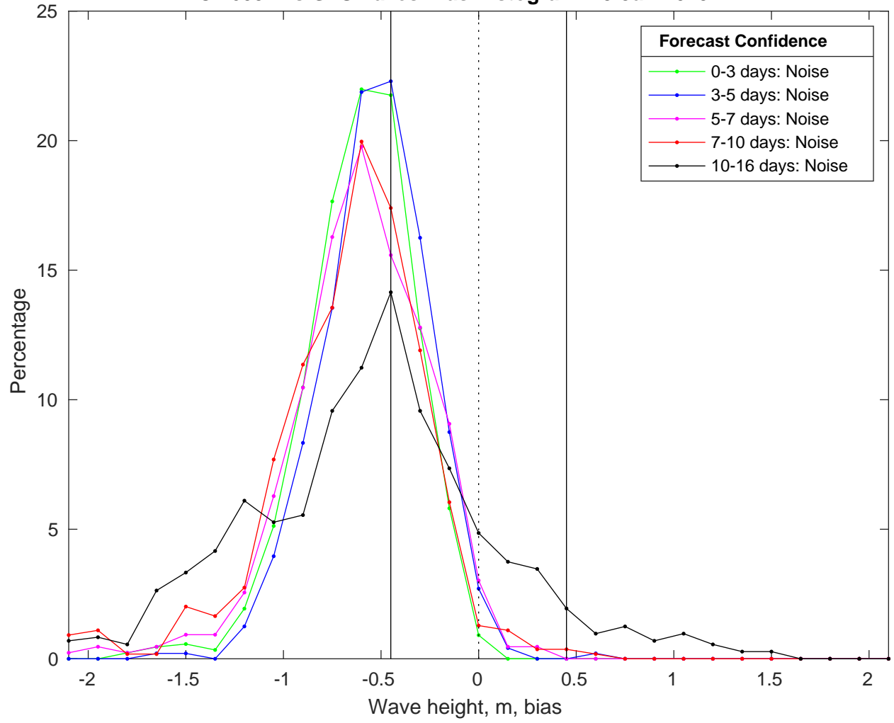
NDBC 46054 vs GFSWaves Bias Histogram: 19-Jan-2025
