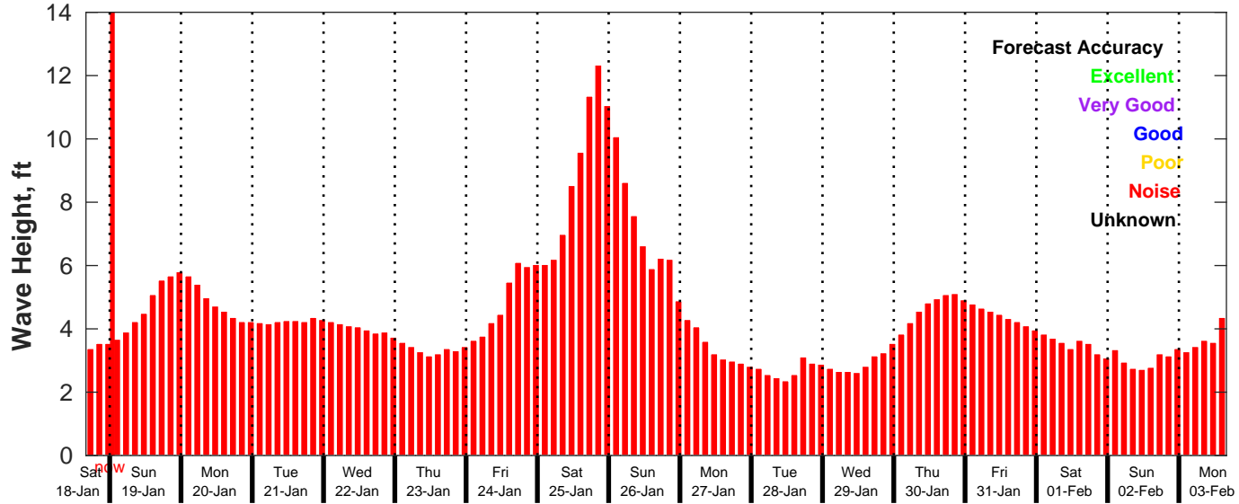
GFS Wave Forecast for NDBC 46054 from 18-Jan-2025 16:00:00 to 03-Feb-2025 16:00:00
